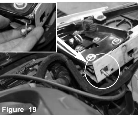
Figure 19 Locate front radiator support hole cut out on passenger side. This will be used to secure the front of heatshield. With provided M6x16 hex screw and fender washer, slide into the cutout.
