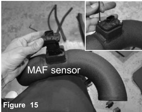
Figure 15 Install the MAF sensor into the new passenger side intake tube. Secure and tighten using 2.5mm allen key.
