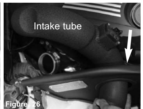
Figure 26 Install the passenger side tube. Position the tube through hole in heat shield and bracket to the vibramount. Install the tube to hose.
