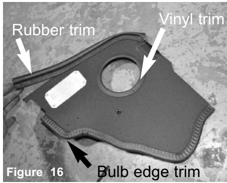
Figure 16 Install the rubber trim to top of the passenger side heat shield. Install the vinyl trim to the hole cut out. Now install the longer bulb edge trim to the bottom of the heat shield.
